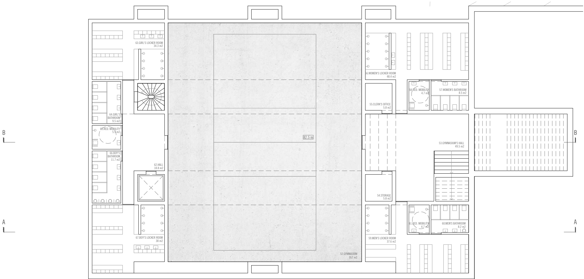
UNDERGROUND PLAN | SCALE 1/200
